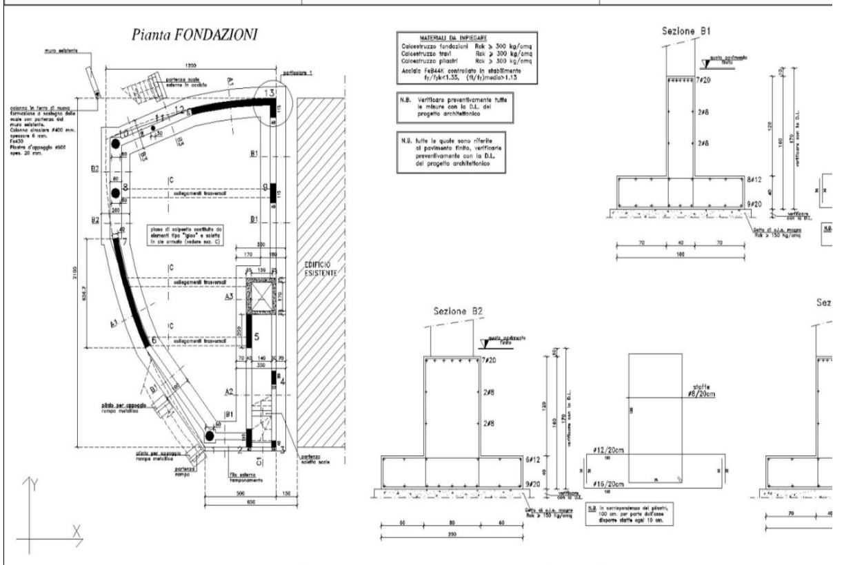
Structural details
