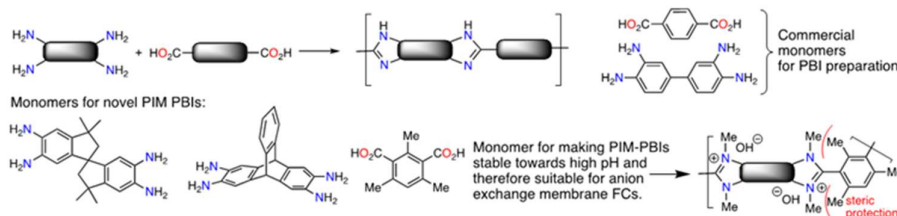
Figure 1: Synthesis of PIMN-PBIs and co polymers from produced monomers
